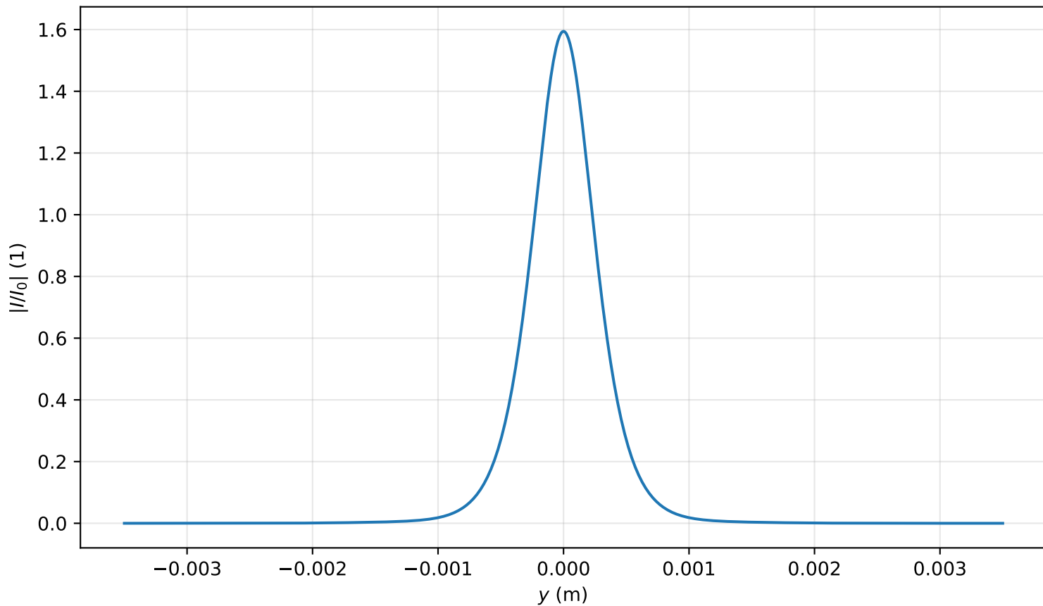
Intensity profile I(x=0, y, z=2.786)/I_0 , P_{in}=0.9P_{cr} , artificial time
